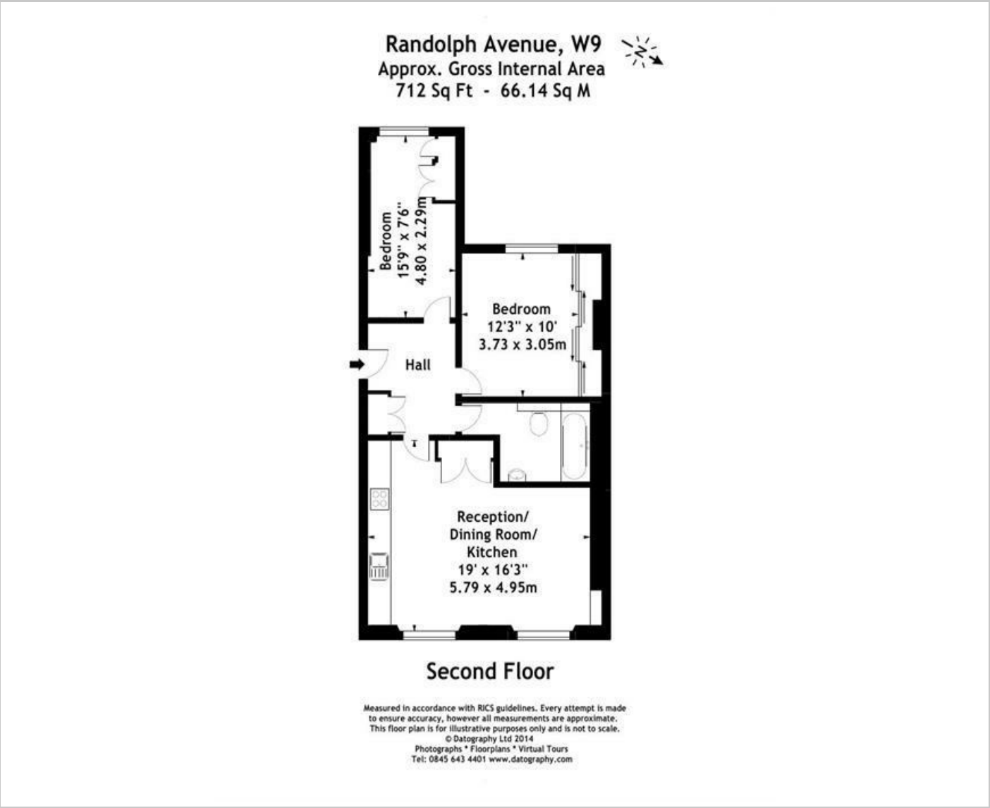
Floor Plan
